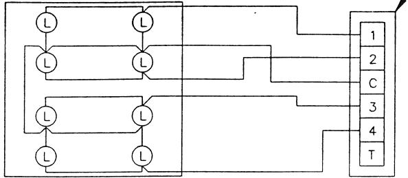
REAR VIEW OF LIGHTBOX SHOWING LAMP CONNECTIONS
