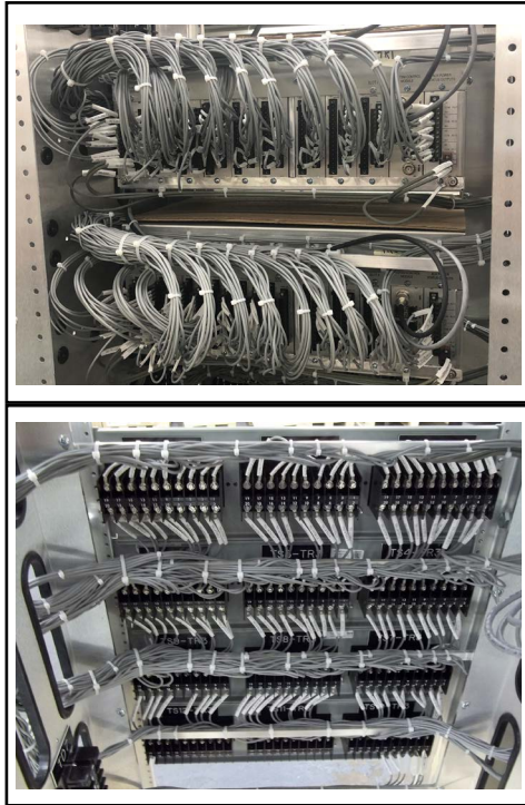
Rear view of Lucasey Rack wiring with TR-3000 and ABB FT-19R test switches.
